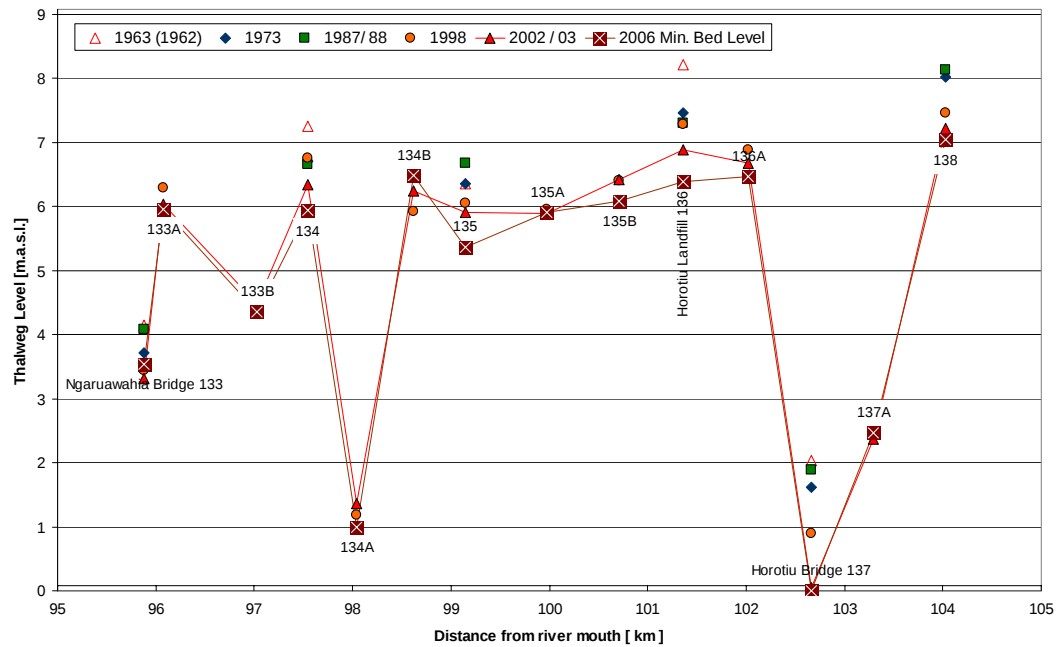
Figure 9 Time evolution of thalweg levels from upstream of Horotiu to Ngaruawahia Bridge
