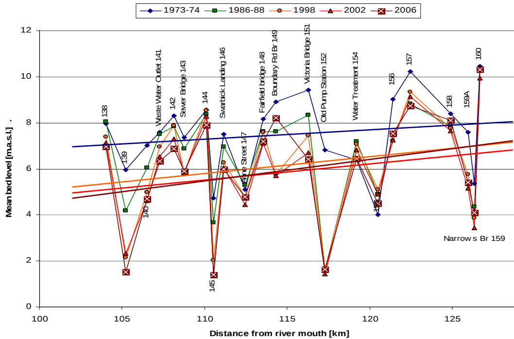
Figure 15 Time evolution of thalweg levels at 22 Hamilton cross-sections. Trendlines show fitted minimum bed level planes.
