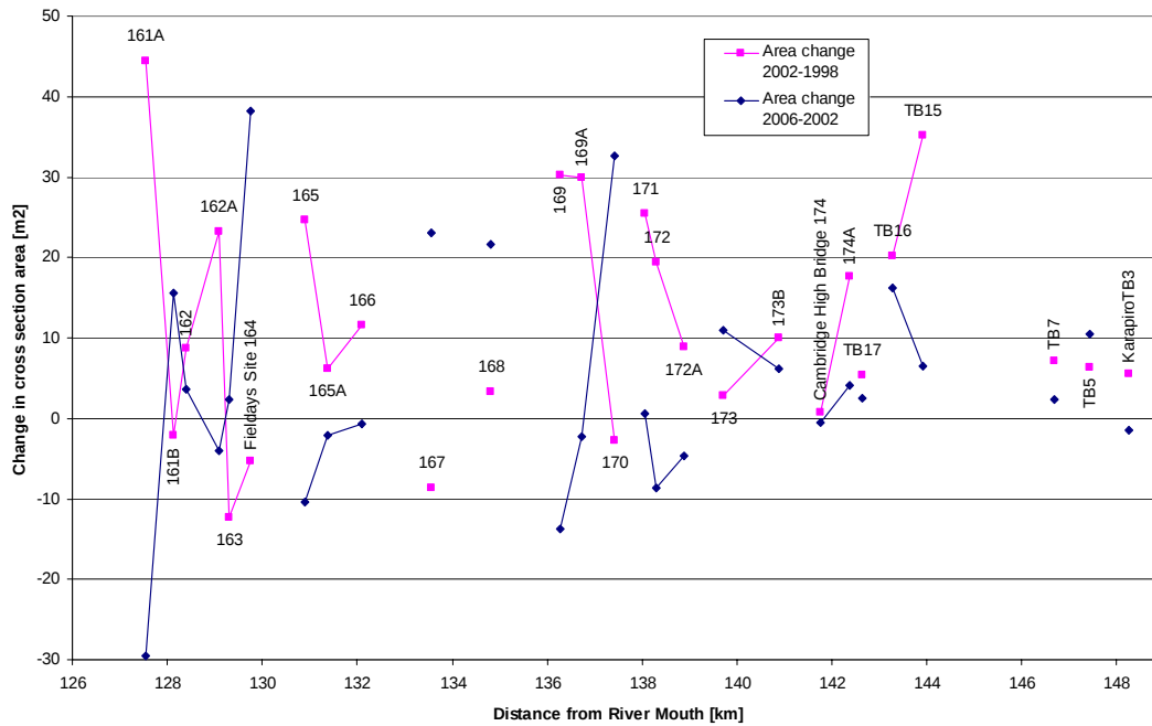
Figure 19 Change in sectional areas between the Narrows and Karapiro ( a positive change indicates scour, a negative change indicates deposition).
