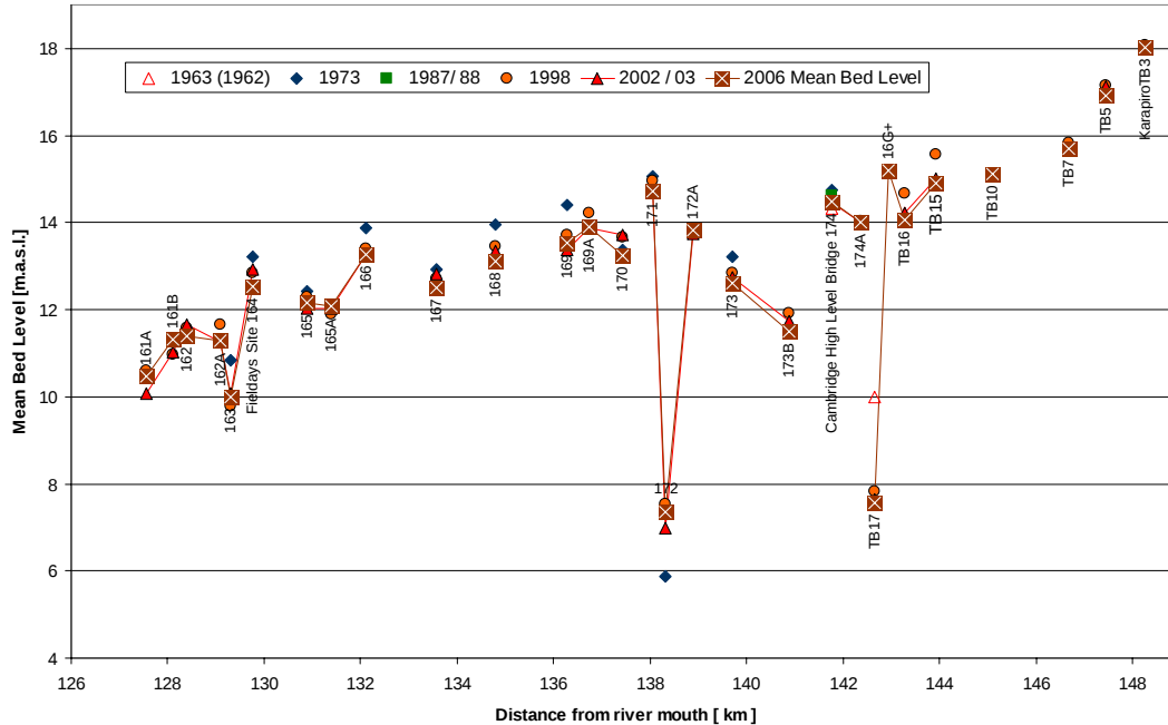
Figure 17 Time evolution of mean bed levels from the tailwater of Karapiro Dam to upstream of The Narrows
