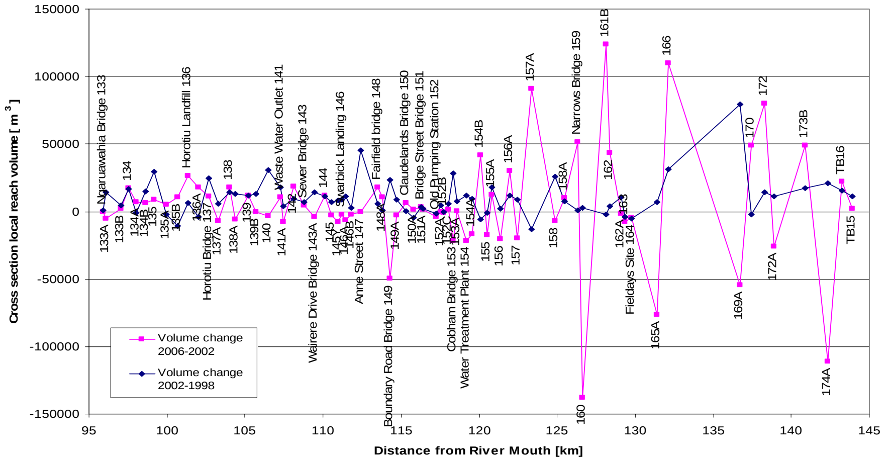
Figure 7 Change in sectional volumes between Karapiro and Ngaruawahia ( a positive change indicates scour, a negative change indicates deposition).
