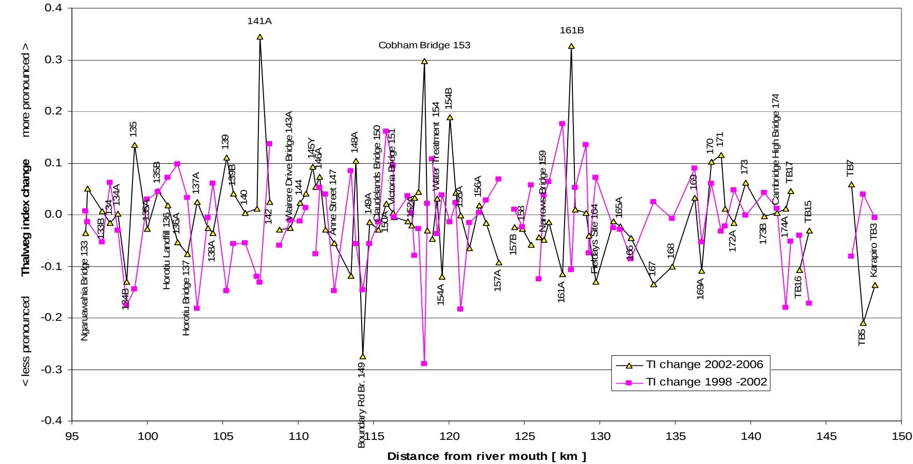
Figure 6 Changes in thalweg significance since 1998
