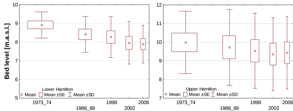
Figure 12 Hamilton City cross section mean bed level statistics from Fairfield Bridge downstream (left) and from Boundary Rd Bridge upstream (right) showing changes with time. SE = standard error, SD = standard deviation of the cross section mean bed level.
