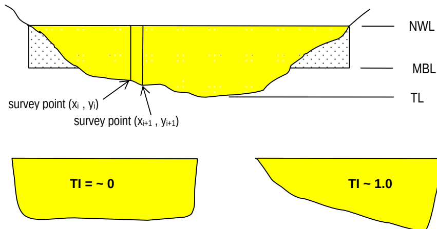
Figure 2 Schematic cross-sections showing Nominal Water Level, Mean Bed Level, Thalweg Level and Thalweg Index.
