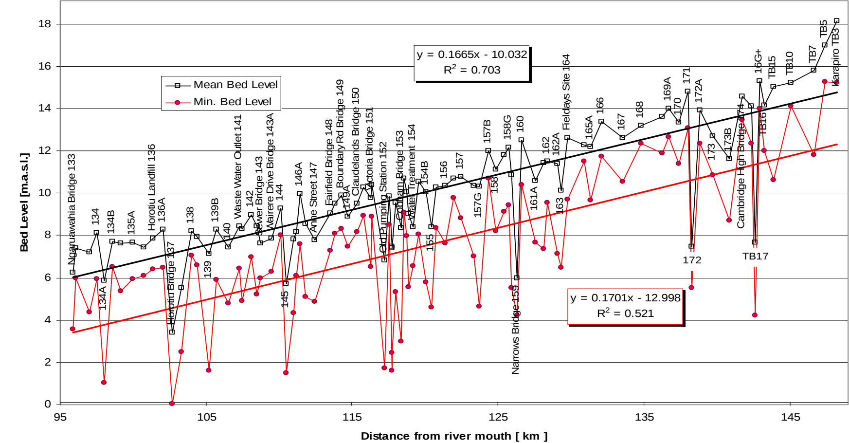
Figure 3 Mean bed levels & thalweg levels from 2006 survey data showing linear trendlines
