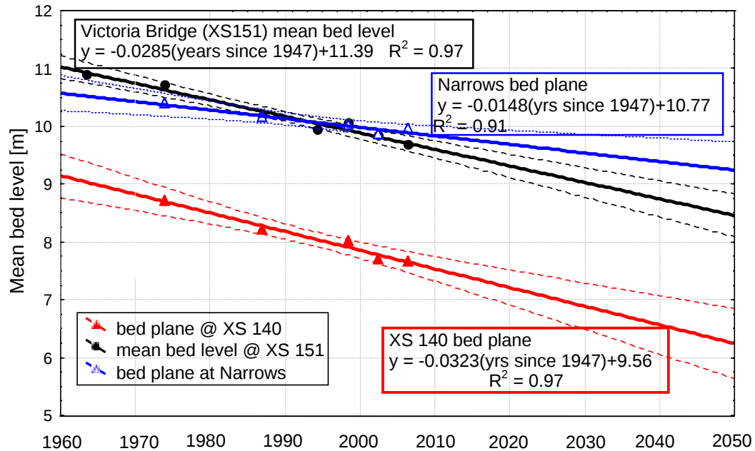
Figure 13 Trends in mean bed level at Victoria St Bridge (Section 151, black line) and trends in level of the bed plane at Pukete Boat Ramp (Section 140, red line) and downstream of Narrows Bridge (km 126, blue line), extrapolated to 2050, showing 95% confidence intervals.
