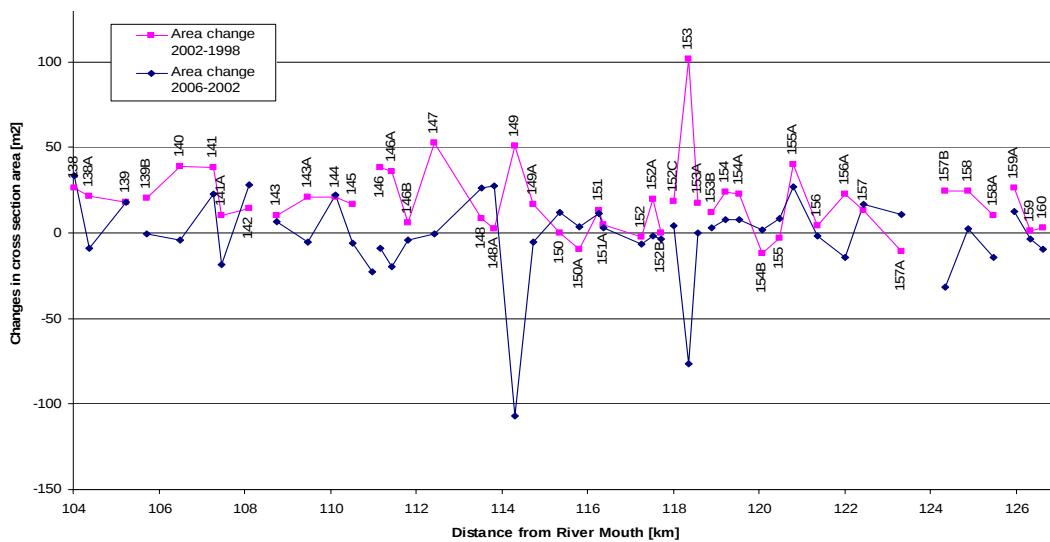
Figure 16 Change in sectional areas for Hamilton reaches (positive change indicates scour, negative change indicates deposition).
