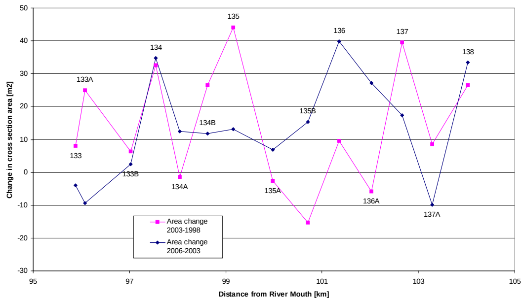
Figure 10 Change in sectional areas from upstream of Horotiu to Ngaruawahia Bridge (a positive change indicates scour, a negative change indicates deposition).
