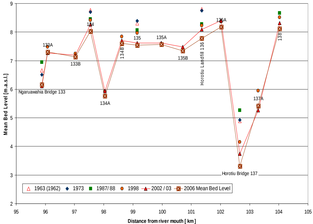
Figure 8 Time evolution of mean bed levels from upstream of Horotiu to Ngaruawahia Bridge
