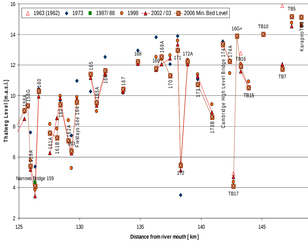
Figure 18 Time evolution of minimum bed levels from the tailwater of Karapiro Dam to upstream of The Narrows.
