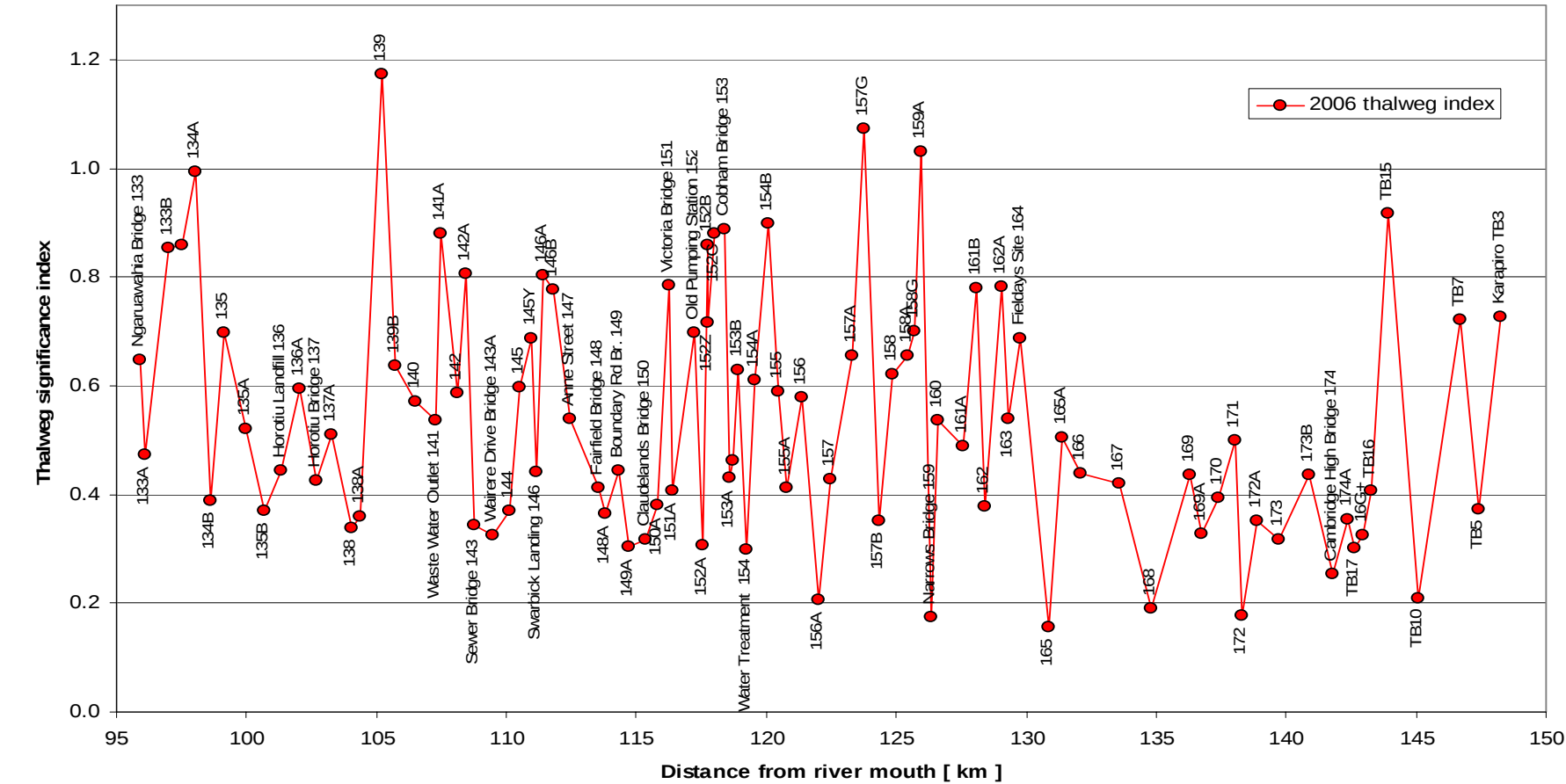
Figure 5 Thalweg significance indicated by 2006 survey
