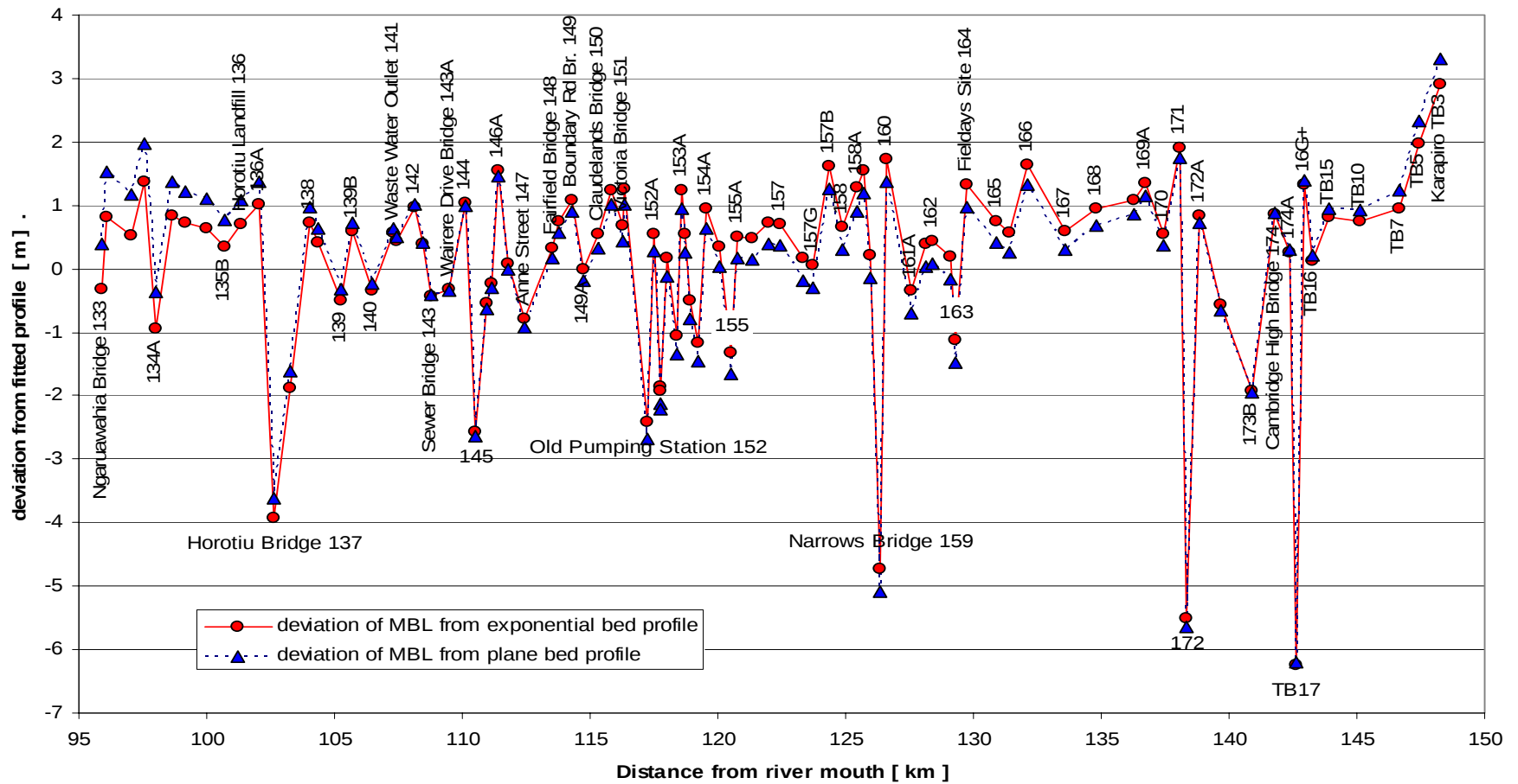
Figure 4 Deviations of mean bed level from fitted profiles using 2006 data.
