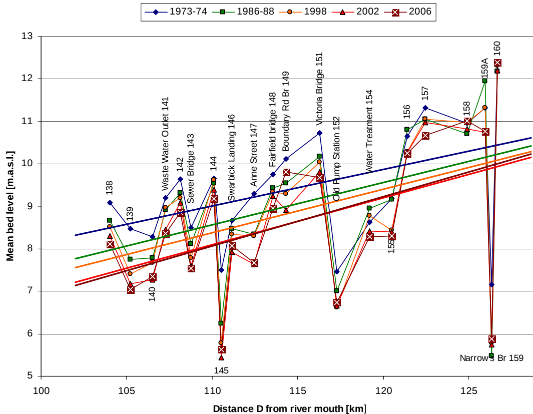
Figure 11 Time evolution of mean bed levels at 22 Hamilton cross-sections. Trendlines show a fitted bed plane.
