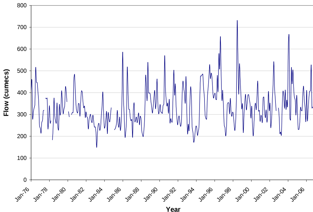
Figure 1 Flow hydrograph for the Waikato River at Hamilton's Victoria Bridge, showing monthly maxima of daily mean flows.
