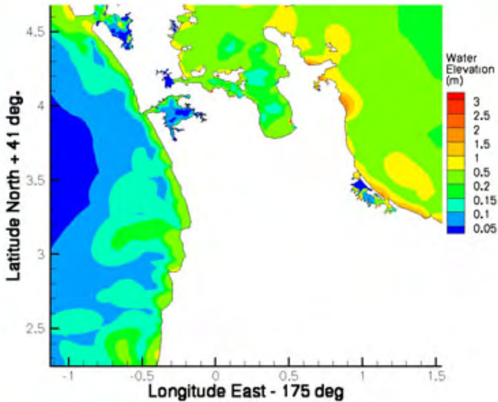
Figure 4.2.3-2: Maximum water surface elevations for the Solomon Sea source with Mw 9.2.
