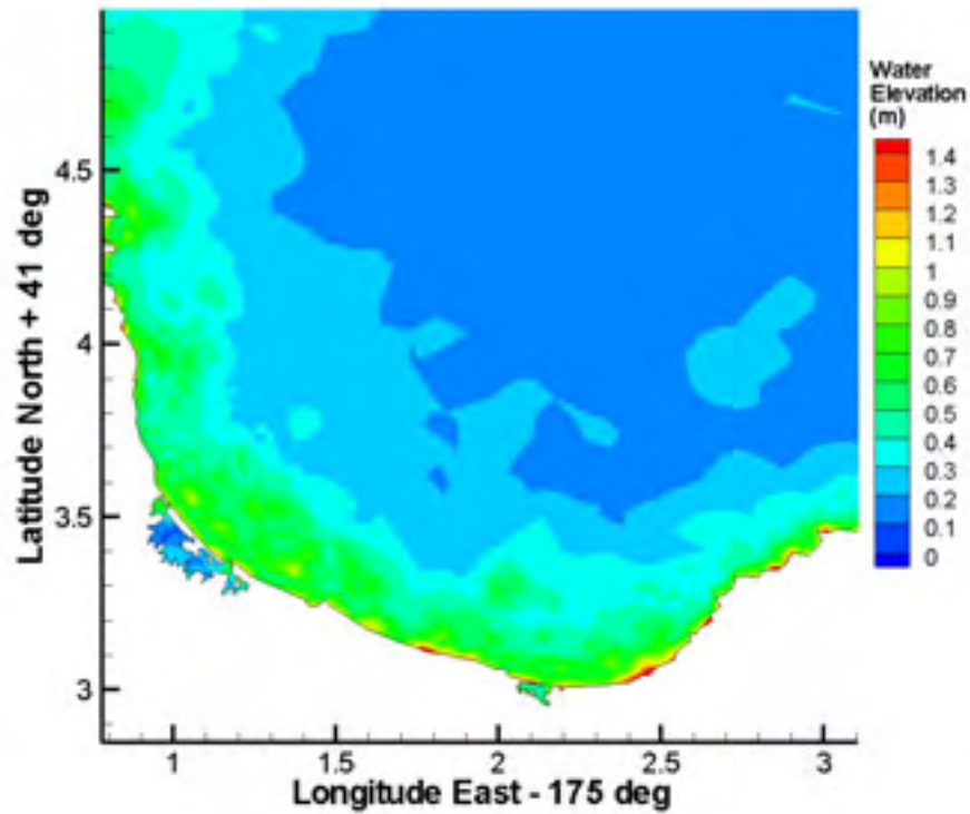
Figure 4.4.3-1: Maximum water surface elevations for the New Hebrides source with Mw 9.2.
