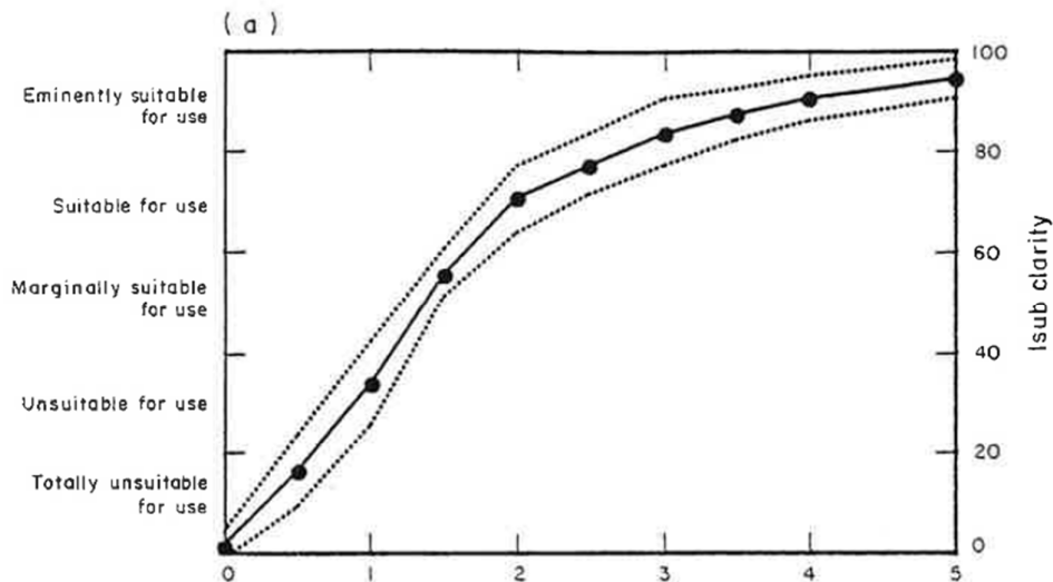
Figure 2. Clarity response curves for bathing. Note: X-axis is Black disc range (m). Reproduced from Smith & Davies-Colley (1992).
