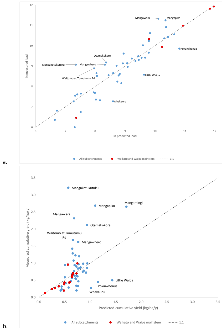
Figure 3-2: Comparison of modelled TP loads and yields against those estimated from measurements. . a. natural log of mean annual TP instream loads; b. mean annual TP cumulative yields. Outliers are labelled
