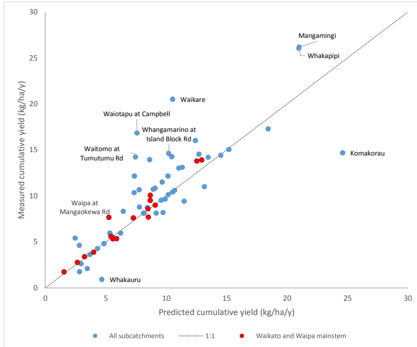
Figure 3-1: Comparison of modelled TN loads and yields against those estimated from measurements. a. natural log of mean annual TN instream loads; b. mean annual TN cumulative yields. Outliers are labelled.
