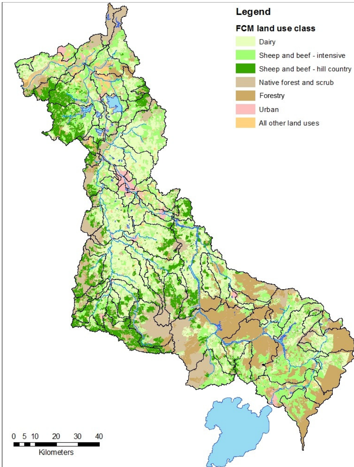
Figure 2-2: Land use from WRC classified into FCM classes. Maize, horticulture and miscellaneous land use classes have been amalgamated for display. Hill country sheep and beef also included a small area of high country sheep and beef.
