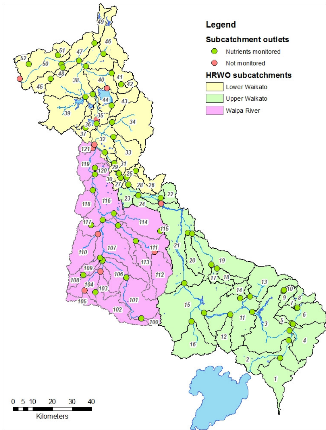
Figure 2-1: Sub-catchments and their associated monitoring sites. Catchment names are listed according to the map reference number in Table 2-2.
