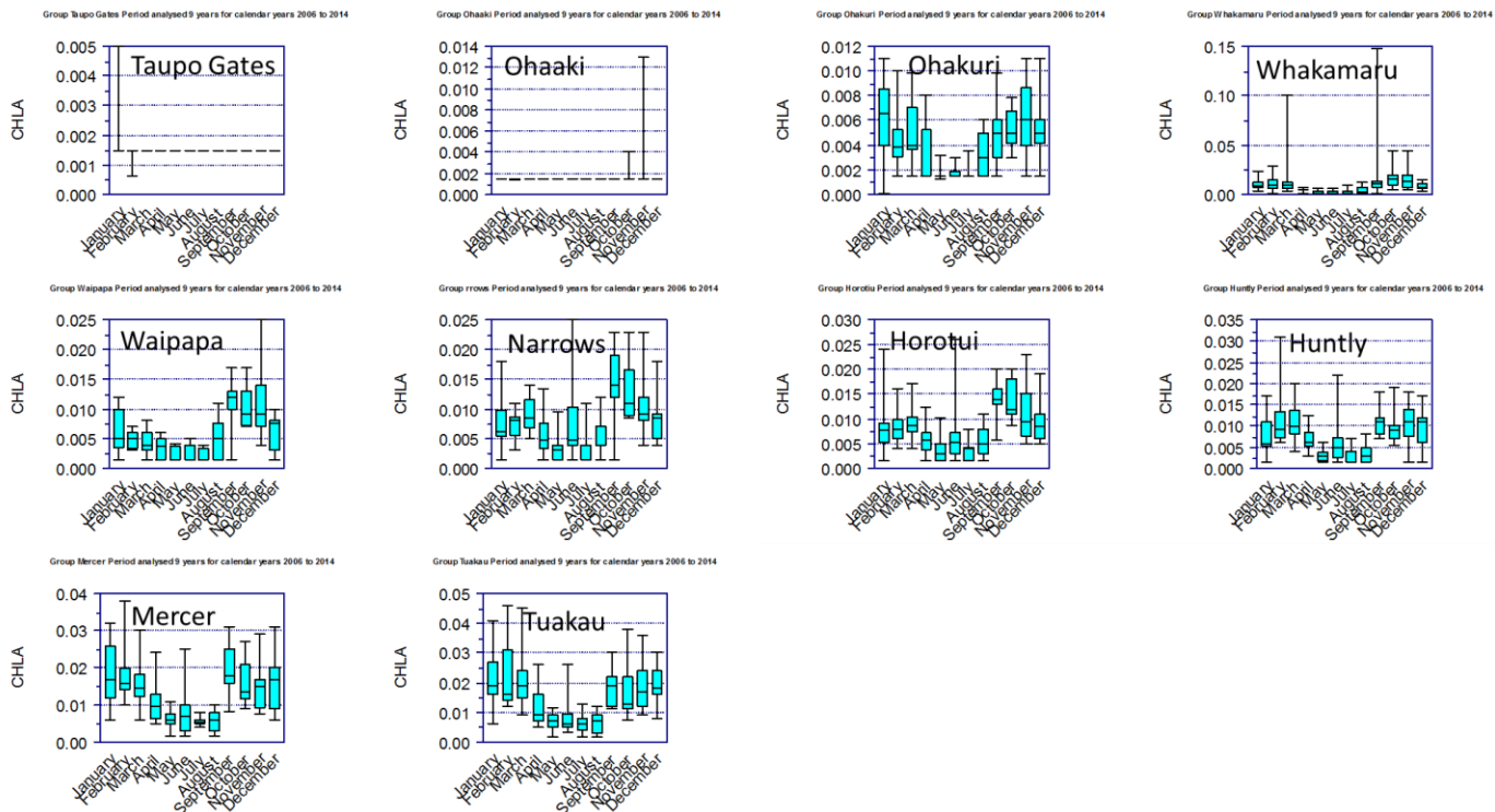
Figure 11: Monthly variations in Chlorophyll a shown as boxplots, 2006-2014. The box represents the 25th-75 th percentile range of the data, the line within the box is the median (50 th percentile) and the whiskers shown the data extremes.
