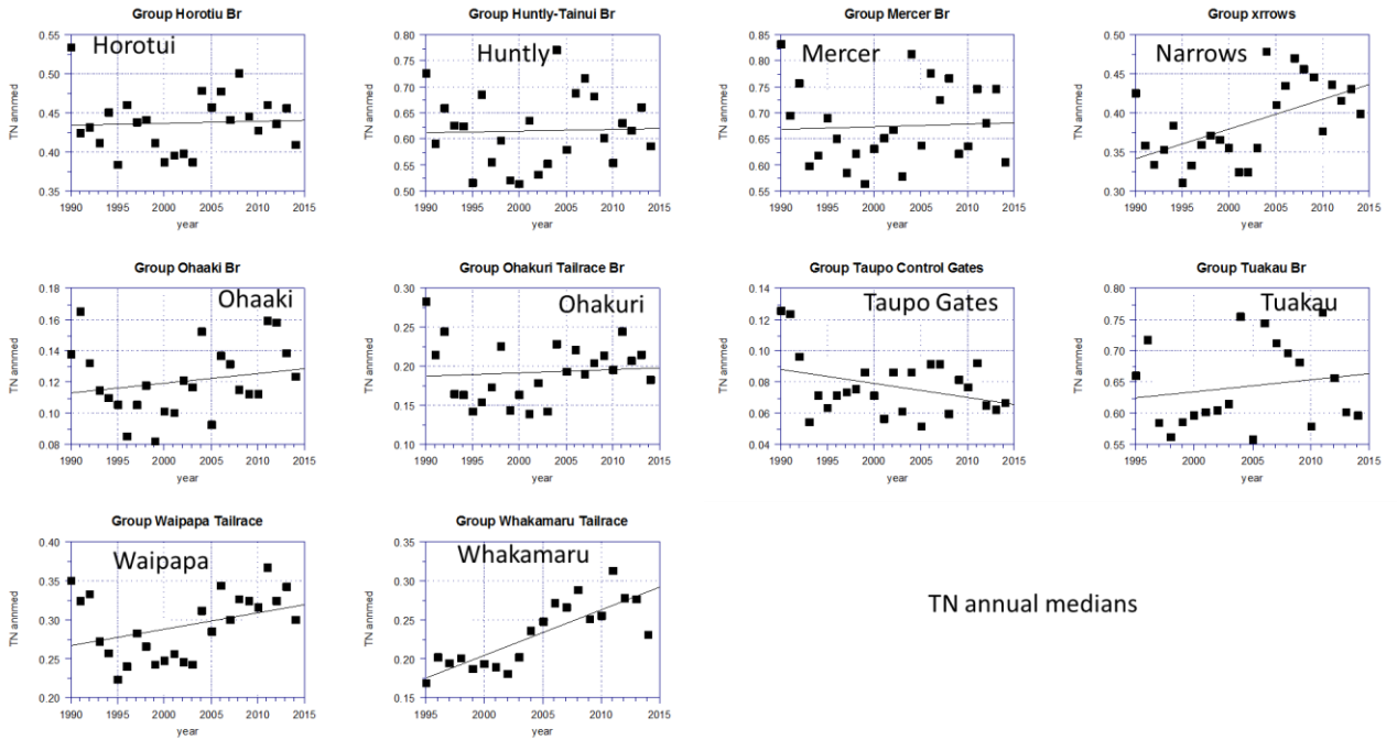
Figure 9: Trends in annual median total nitrogen ( \text{g}/\text{m}^3 ) over 1990-2014 at Waikato main stem sites.
