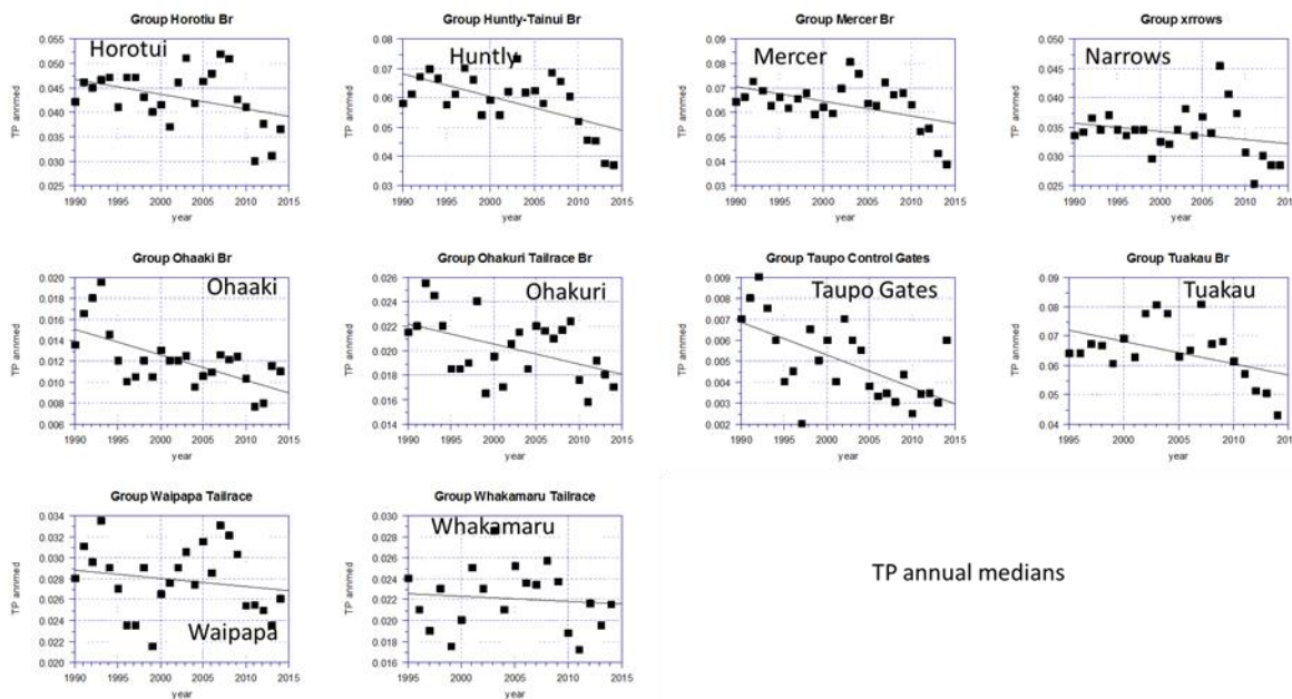
Figure 8: Trends in annual median total phosphorus ( \text{g/m}^3 ) over 1990-2014 at Waikato mainstem sites.
