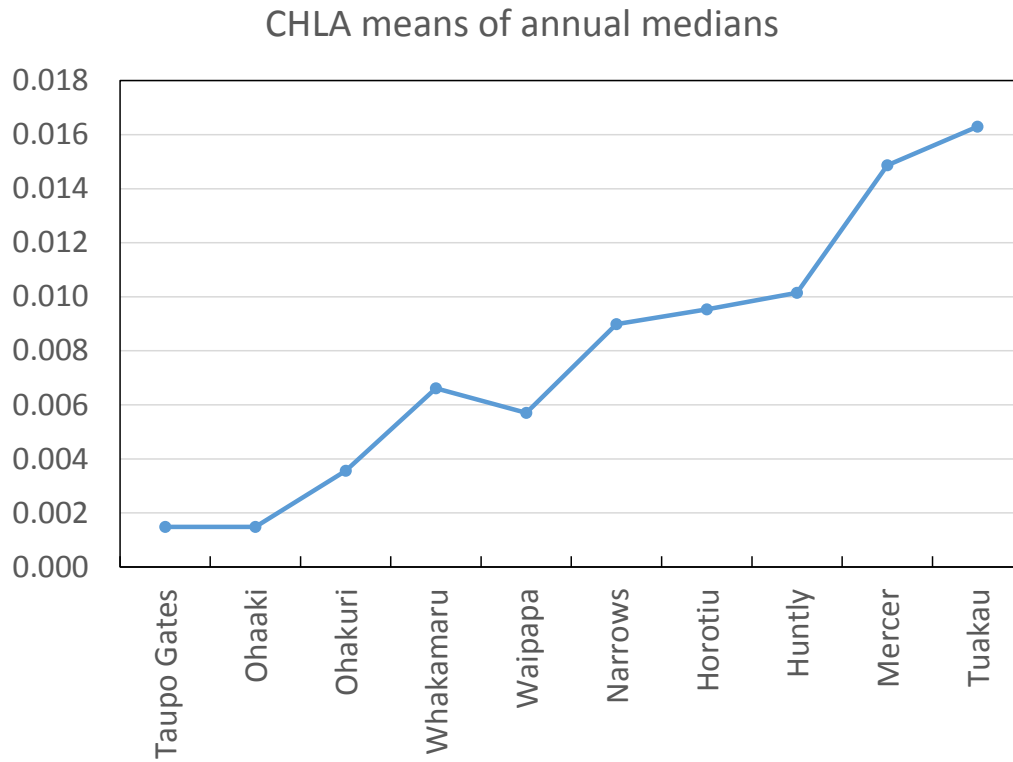
Figure 1: Spatial variation in median chlorophyll a (g/m 3 ) along the Waikato main stem (1990-2014).
