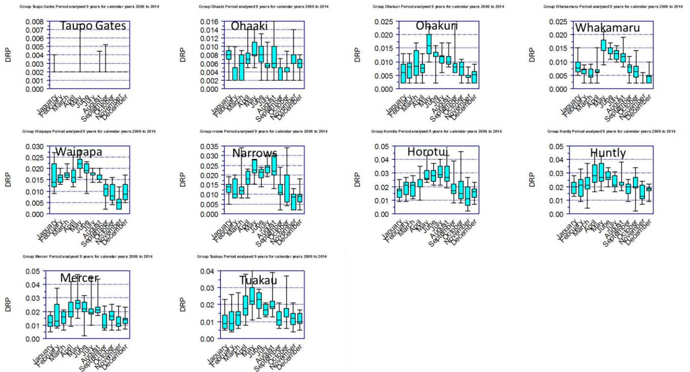
Figure 13: Monthly variations in dissolved reactive phosphorus as boxplots, 2006-2014.
