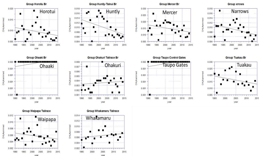
Figure 7: Trends in annual median chlorophyll a ( \text{g/m}^3 ) over 1990-2014 at Waikato main stem sites. NB Whakamaru data are unreliable.
