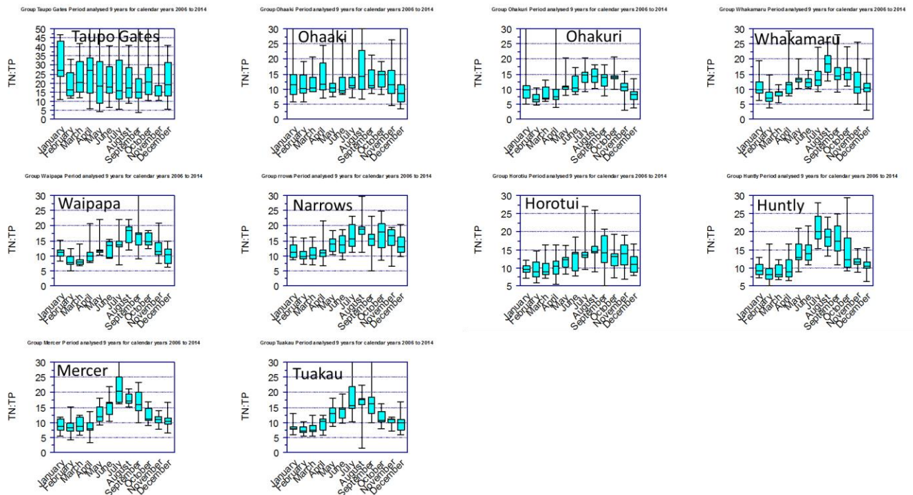
Figure 14: Monthly variations in TN:TP as boxplots, 2006-2014.
