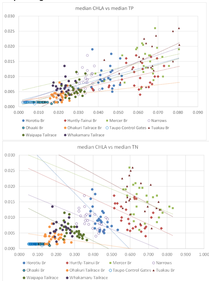
Figure 6: Relationships at each site between annual median Chl. a and TN and TP (all g/m^3 ) at Waikato main stem sites 1990-2014 (from 1995 for Tuakau and Whakamaru) showing regression lines for individual sites (excluding Whakamaru, Ohaaki, Taupo Gates).
