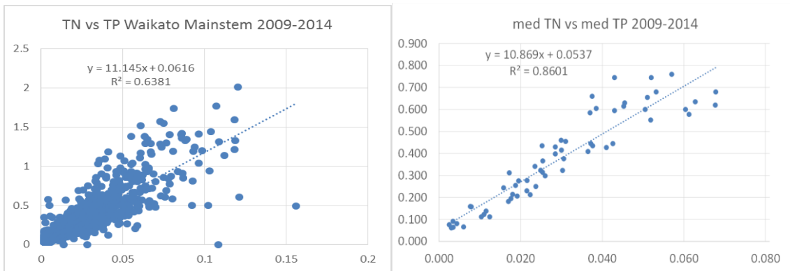
Figure 5: Relationships TN and TP across Waikato Mainstem sites below Arapuni 2009-2014 for all data and annual medians.
