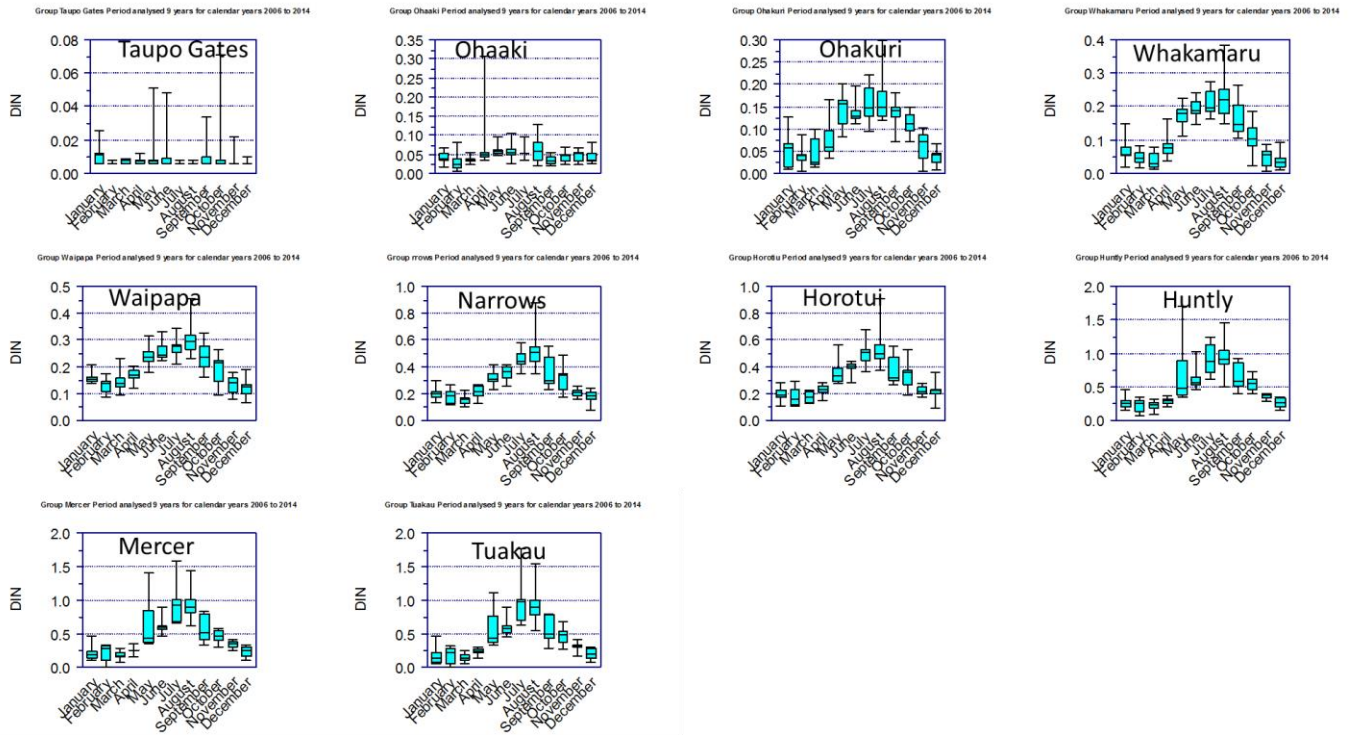
Figure 12: Monthly variations in dissolved inorganic N as boxplots, 2006-2014.
