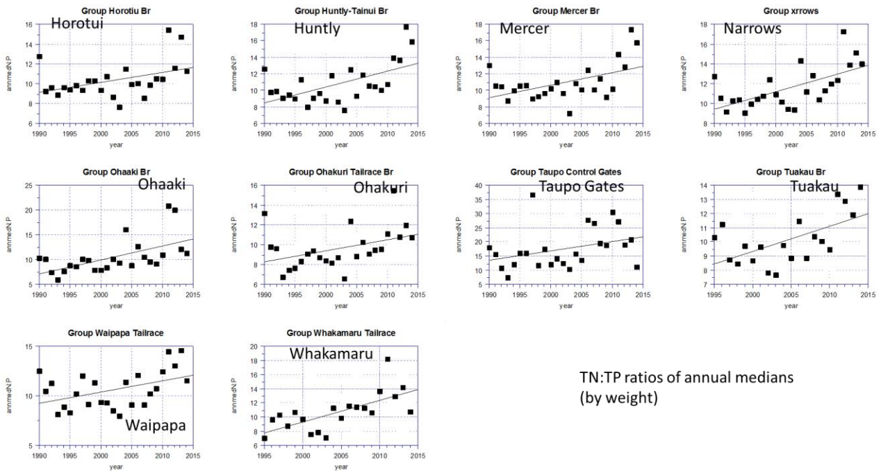
Figure 10: Trends in annual median TN/TP over 1990-2014 at Waikato main stem sites.
