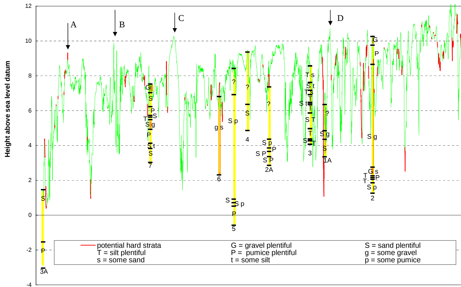
Figure 10 Thalweg (green) between Horotiu and the Narrows showing initial borehole logs relative to potential hard strata (red). Borehole numbers are below the holes. Yellow strata are easily erodable, orange contain gravel. High sills are indicated by arrows.
