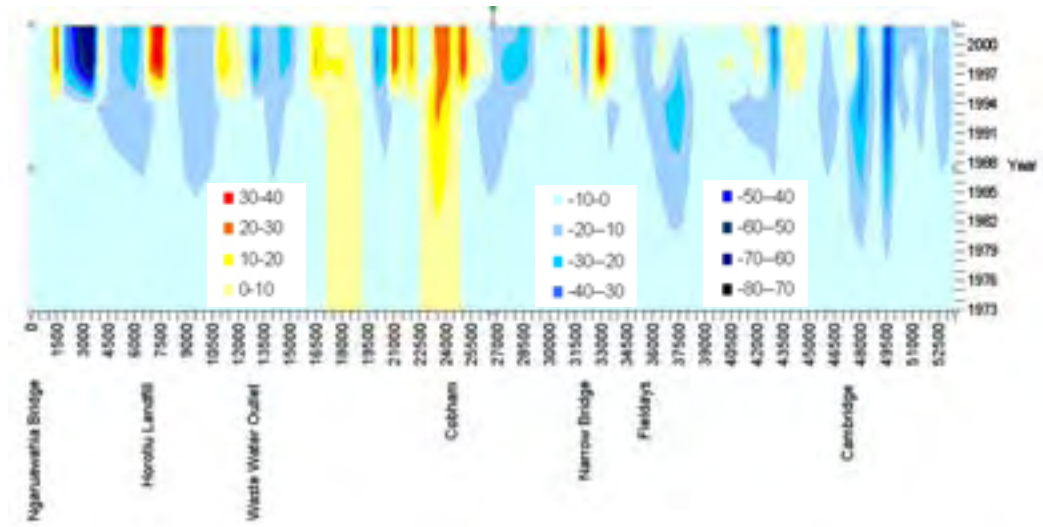
Figure 5. Changes in width of an average annual flood from Ngaruawahia Bridge to Karapiro between 1973 and 2003 (yellow, orange and red indicate widening up to 40 m, darker blue regions show narrowing of up to 80m). Ref. EWDOCS-#923799.
