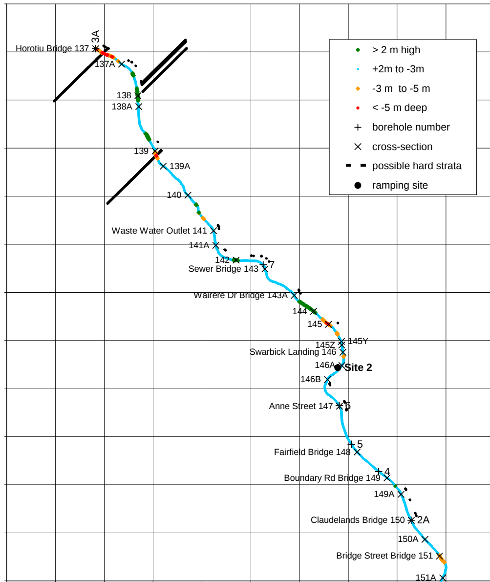
Figure 2 Bed levels of Northern Hamilton reaches, indicated by deviation of the thalweg elevation from its linear trend line. Possible hard strata, cross-sections and borehole measurement locations are shown. Grid size is 1km.
