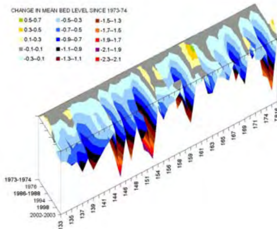
Figure 1 Changes in mean bed level since 1973, shown in metres, from Section 133 (near Ngaruawahia) to Section TB16 (near Karapiro Dam).
