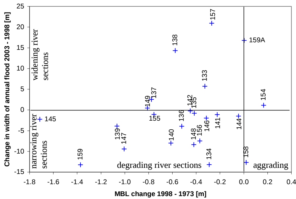
Figure 8 Changes in mean bed level between 1973 and 1998 and changes in annual flood width between 1998 and 2003 for sections between Ngarauwahia and the Narrows.
