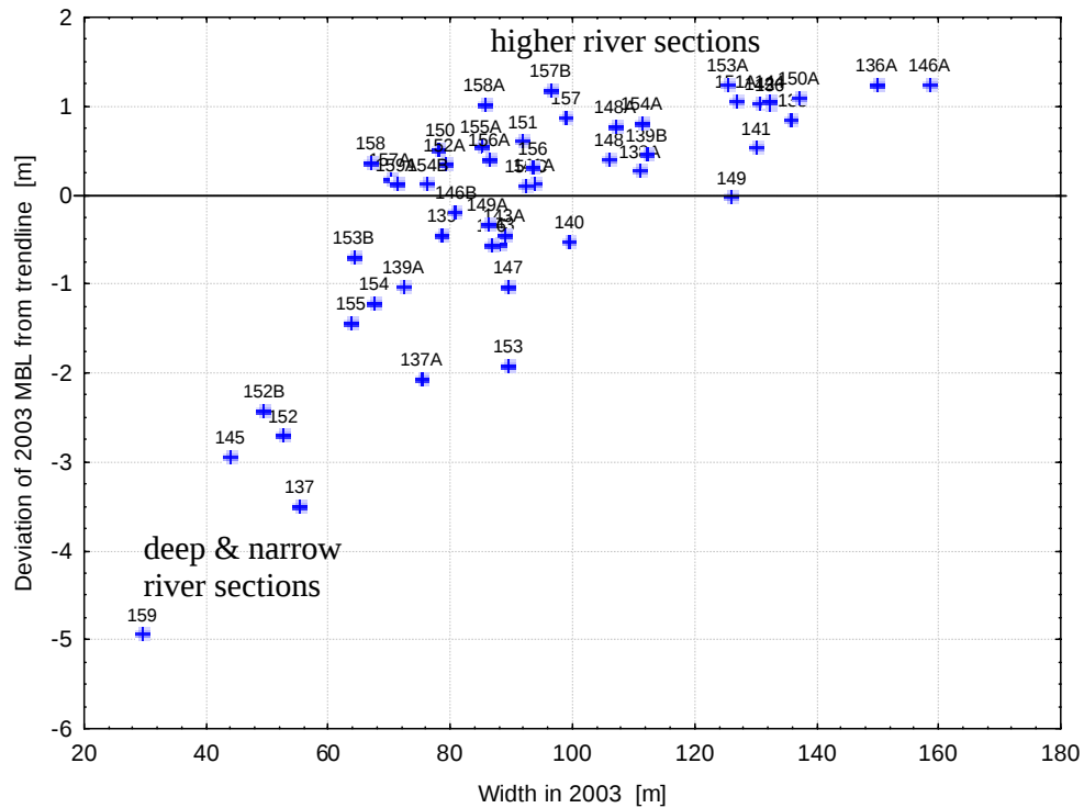
Figure 7 Deviation of mean bed level from its trend line and flood width for the 2003 survey data, Horotiu Landfill to Narrows Bridge cross sections.
