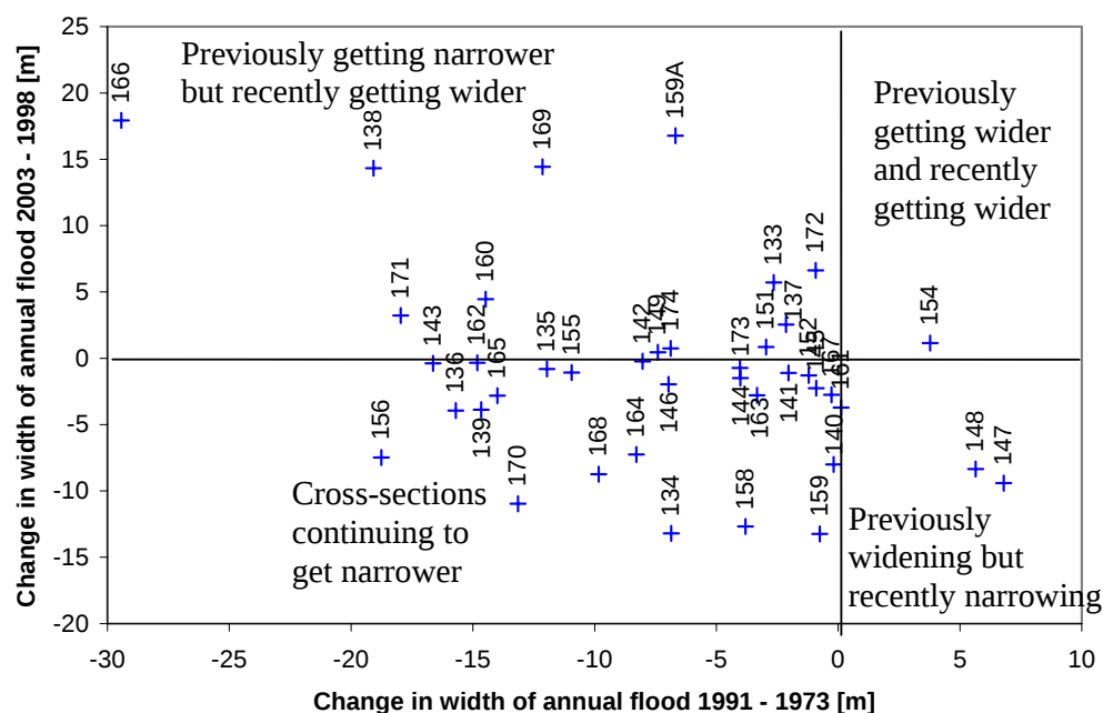
Figure 9 Comparison of recent width changes with past width changes.
