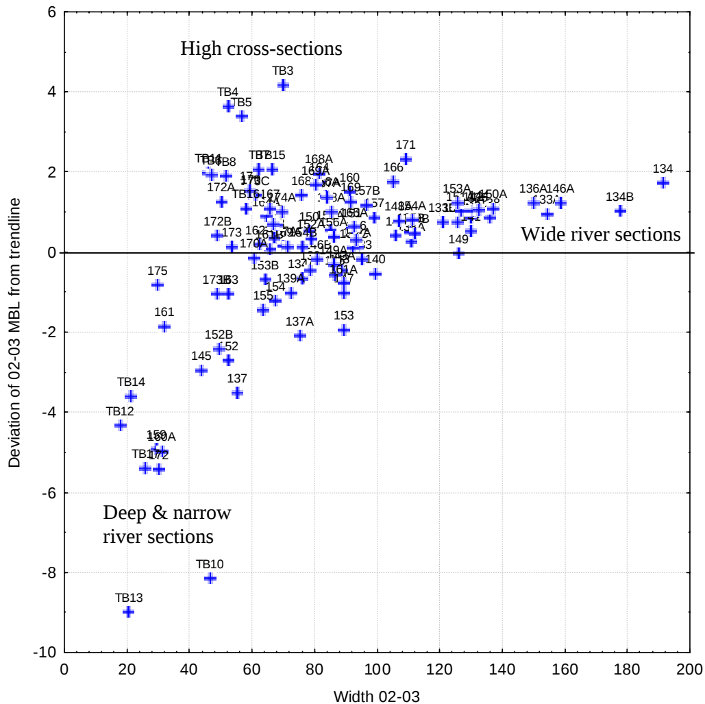
Figure 6 Deviation of Mean Bed Level from its trendline and flood width for the 2003 survey data, Ngaruawahia to Karapiro.
