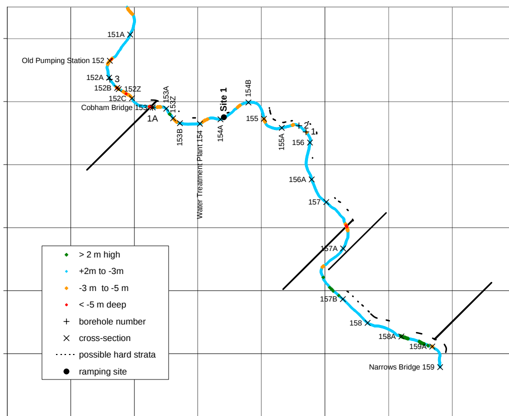
Figure 3 Bed levels of Southern Hamilton reaches, indicated by deviation of the thalweg elevation from its linear trend line. Possible hard strata, cross-sections and borehole measurement locations are shown. Grid size is 1km.
