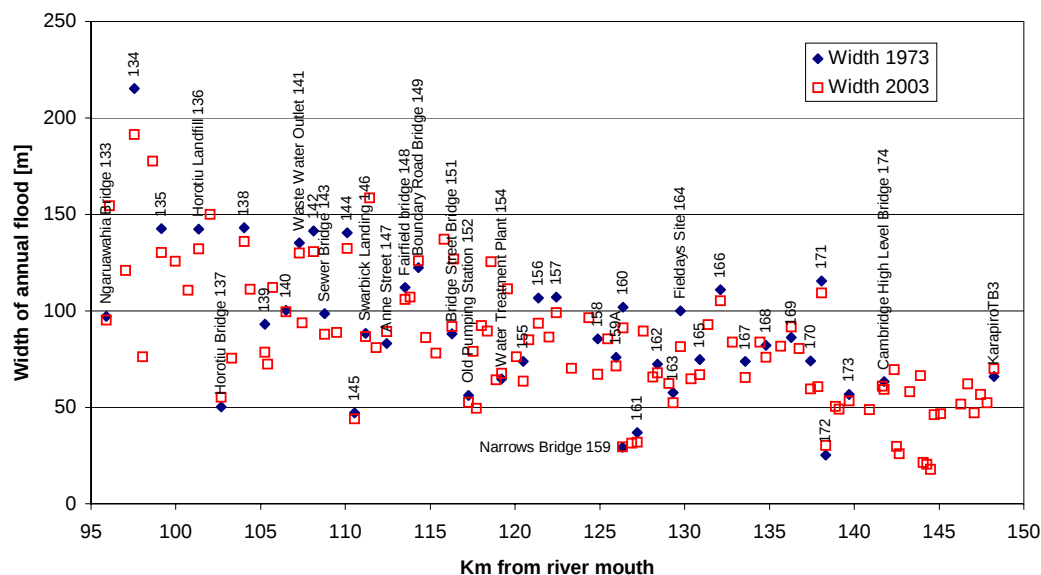
Figure 4 Profile of flood widths from Ngaruawahia to Karapiro in 1973 and 2003.
